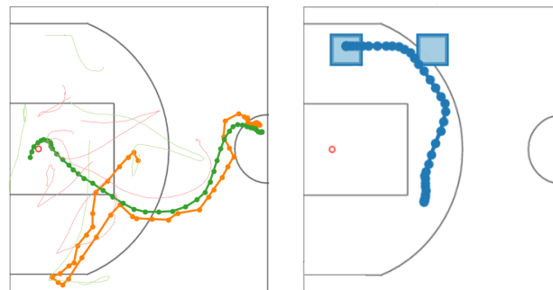
(a) Two player (green) macro-goals: 1) pass the ball (orange) 2) move to the basket. (b) Depicting two spatial macro-goals (blue boxes) as an agent moves to the top left.
