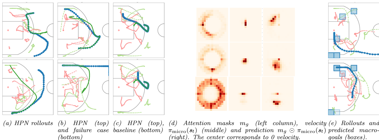
Figure 3: Rollouts (columns a, b, c). Each frame shows an offensive player (dark green), a rollout (blue) track that extrapolates after 20 frames, the offensive team (light green) and defenders (red). Note we do not show the ball, as we did not use semantic basketball features (i.e. “currently has the ball”) during training. The HPN rollouts do not memorize training tracks (column a) and display a variety of natural behavior, such as curving and making sharp turns. We also show a failure case (b, bottom): the HPN moves along a straight line off the right border, which may be fixable by using extra game state information. For comparison, a hierarchical baseline without attention, produces a straight-line rollout (column b, bottom), whereas the HPN produces a more natural movement curve (column c, top). Attention model (column d). Visualizing how the attention m_g interacts with the micro-planner \pi_{\text{micro}} . Row 1: \pi_{\text{micro}} decides to stay still, but the attention m_g wants to go left. The weighted result m_g \odot \pi_{\text{micro}}(s_t) moves to the top-left, with an average speed. Row 2: \pi_{\text{micro}} wants to go down, while m_g boosts the velocity so the agent bends to the bottom-left. Row 3: \pi_{\text{micro}} remains stationary, but m_g prefers to move in any direction. As a result, the agent moves down. Macro-goals (column e). The HPN dynamically predicts macro-goals and guides the micro-planner in order to reach them. Box intensity corresponds to relative prediction frequency during the trajectory. The macro-goal predictions are stable over a large time horizon. The HPN sometimes predicts inconsistent macro-goals, e.g. in the bottom right frame, the agent moves to the top-left, but sometimes predicts the macro-goal to be in the bottom-left.
